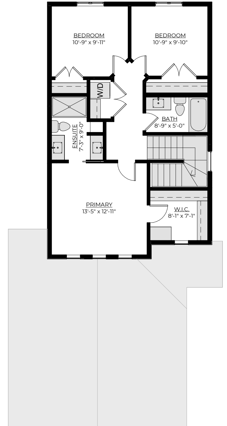
Second Floor Plan 811 ft 2
